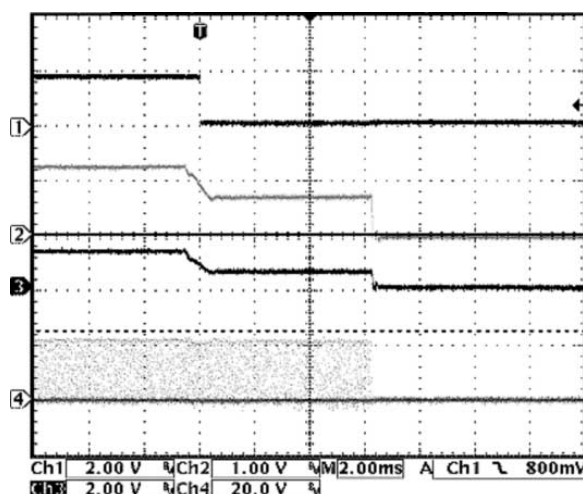
Figure 2. Overcurrent Latch-Off Waveforms, Circuit of Figure 4. Channel 1—PWRGD, Channel 2— V_{\text{OUT}} , Channel 3—CSCOMP Pin of ADP3168, Channel 4—High-Side MOSFET V_{\text{GS}}
