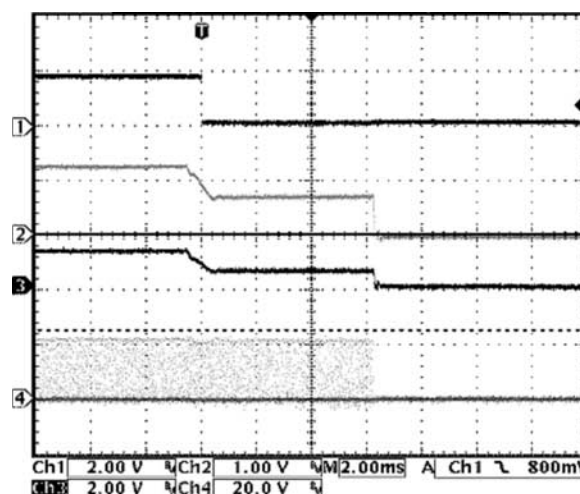
Figure 2. Overcurrent Latch-Off Waveforms, Circuit of Figure 4. Channel 1–PWRGD, Channel 2– V_{\text{OUT}} , Channel 3–CSCOMP Pin of ADP3180, Channel 4–High Side MOSFET V_{\text{GS}}
