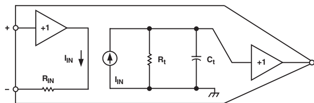
Figure 1. Equivalent Schematic
