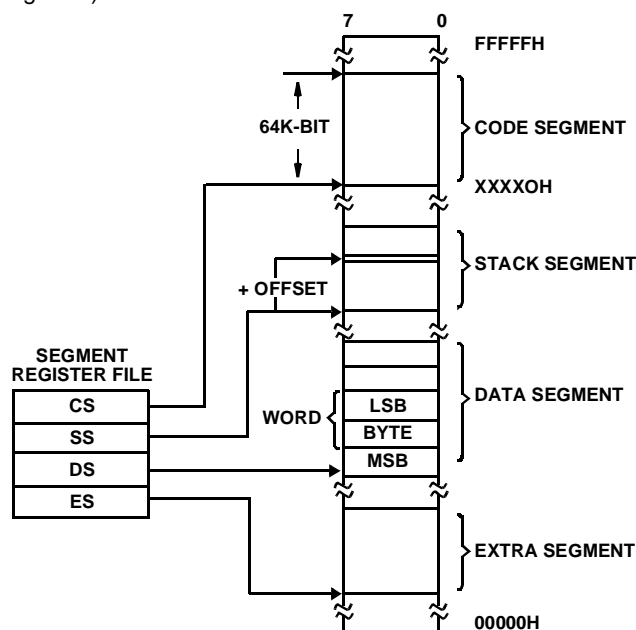
FIGURE 14. MEMORY ORGANIZATION
