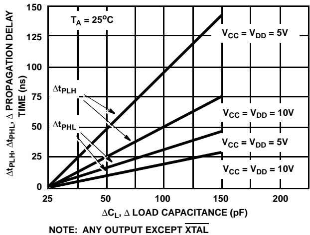
FIGURE 22. TYPICAL CHANGE IN PROPAGATION DELAY AS A FUNCTION OF A CHANGE IN LOAD CAPACITANCE FOR ALL TYPES
