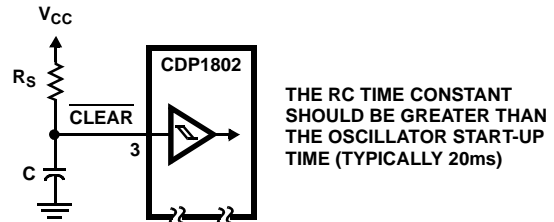
FIGURE 24. RESET DIAGRAM
