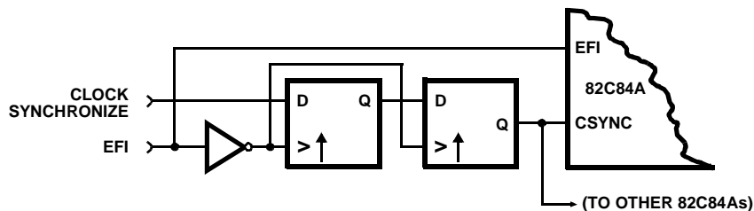
FIGURE 1. CSYNC SYNCHRONIZATION
