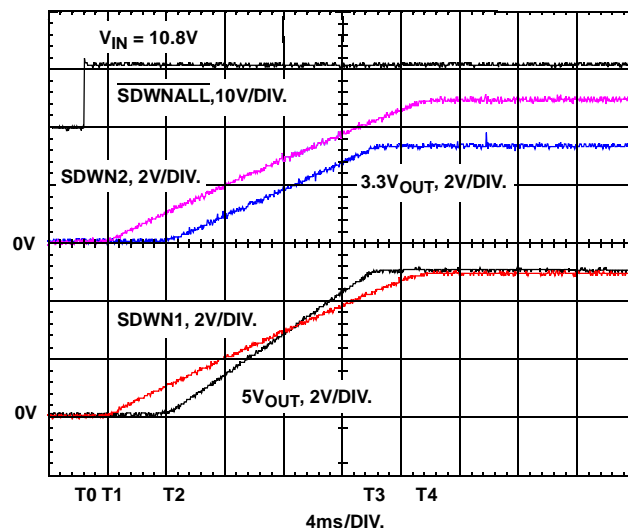
FIGURE 2. SOFT START ON 3.3V AND 5V OUTPUTS
