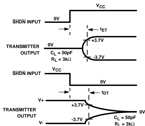
FIGURE 2. TRANSMITTER OUTPUT ENABLE AND DISABLE TIMING
