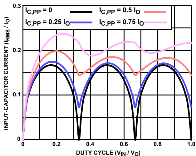
FIGURE 16. NORMALIZED INPUT-CAPACITOR RMS CURRENT VS DUTY CYCLE FOR 3-PHASE
