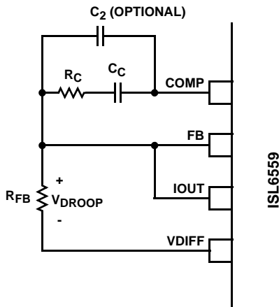
FIGURE 12. COMPENSATION CONFIGURATION FOR LOAD-LINE REGULATED ISL6559 CIRCUIT
