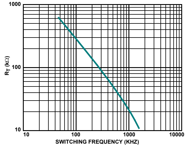
FIGURE 14. R_T VS SWITCHING FREQUENCY
