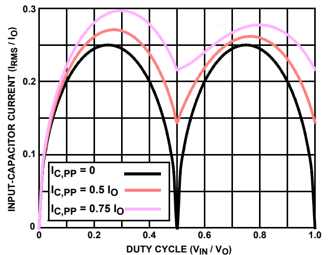
FIGURE 15. NORMALIZED INPUT-CAPACITOR RMS
