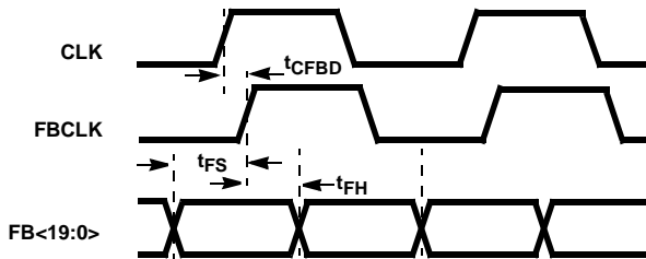
FIGURE 19. FEEDBACK TIMING
