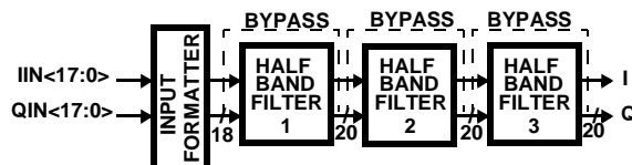
FIGURE 2. INPUT FORMATTER AND INTERPOLATOR BLOCK DIAGRAM
