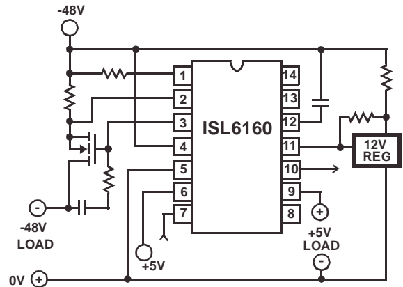
FIGURE 3. -48V/+5V APPLICATION CIRCUIT
