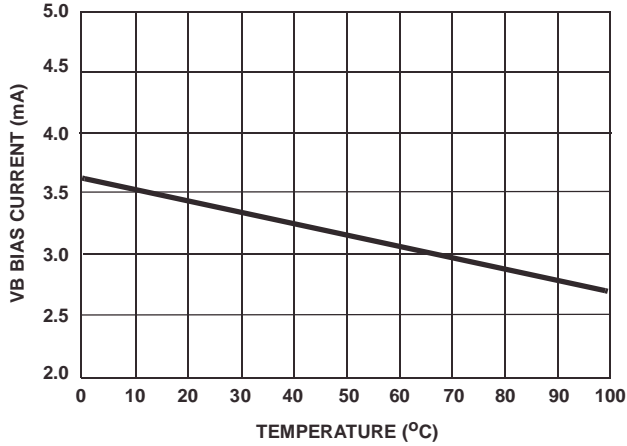
FIGURE 5. VB BIAS CURRENT
