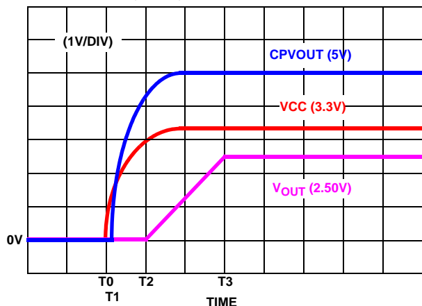
FIGURE 1. SOFT-START INTERVAL
