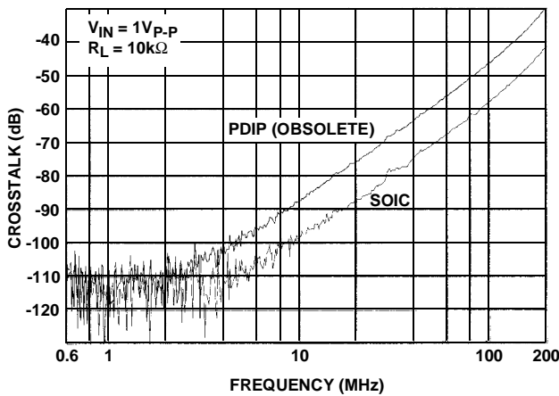
FIGURE 7. ALL HOSTILE CROSSTALK REJECTION
