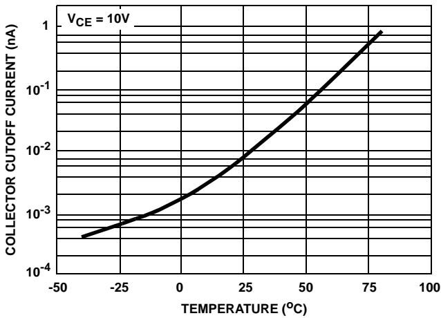
FIGURE 19. I_{CBO} vs TEMPERATURE FOR ANY TRANSISTOR
