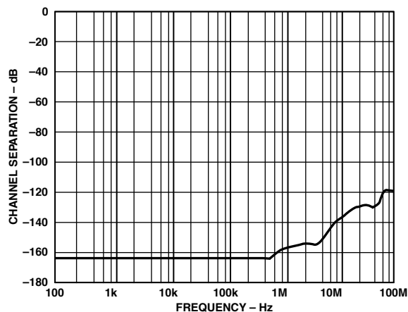
Figure 4. Channel Separation vs. Frequency
