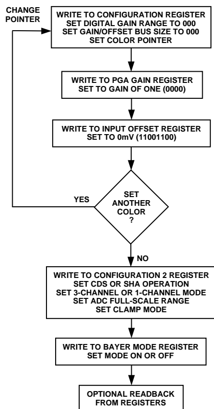
Figure 19. Initialization
