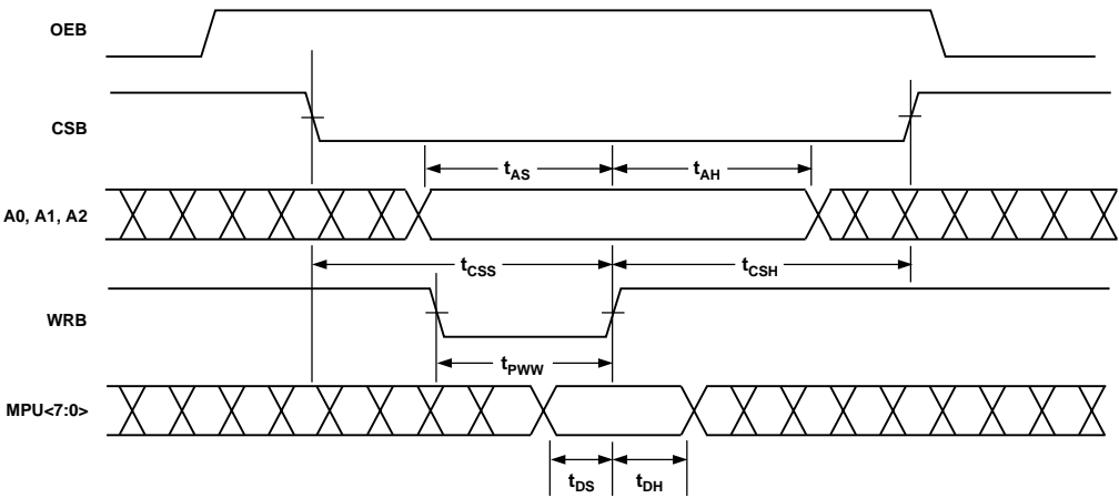
Figure 2. Write Timing
