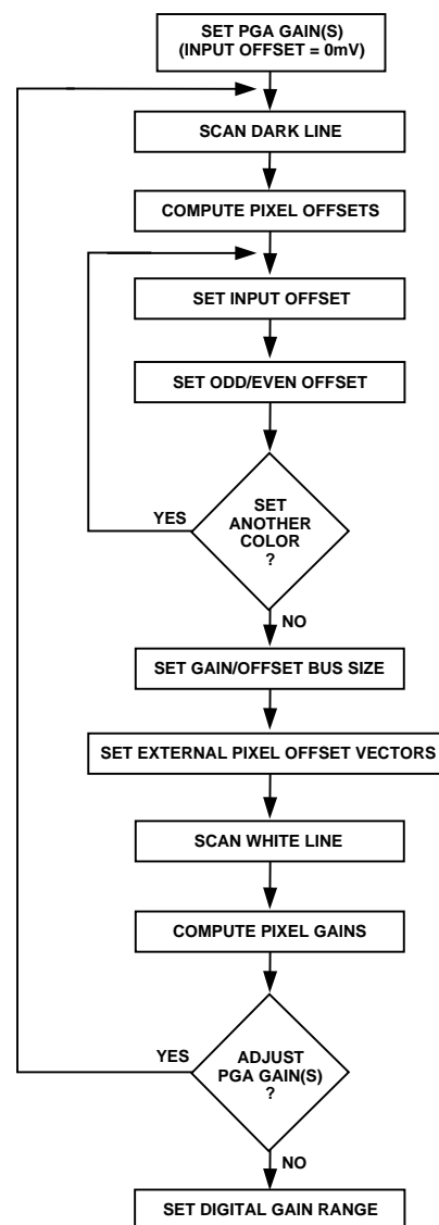
Figure 20. Calibration
