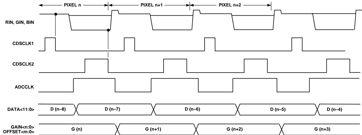
Figure 14. DOUT Latency, 1-Channel CDS Mode
