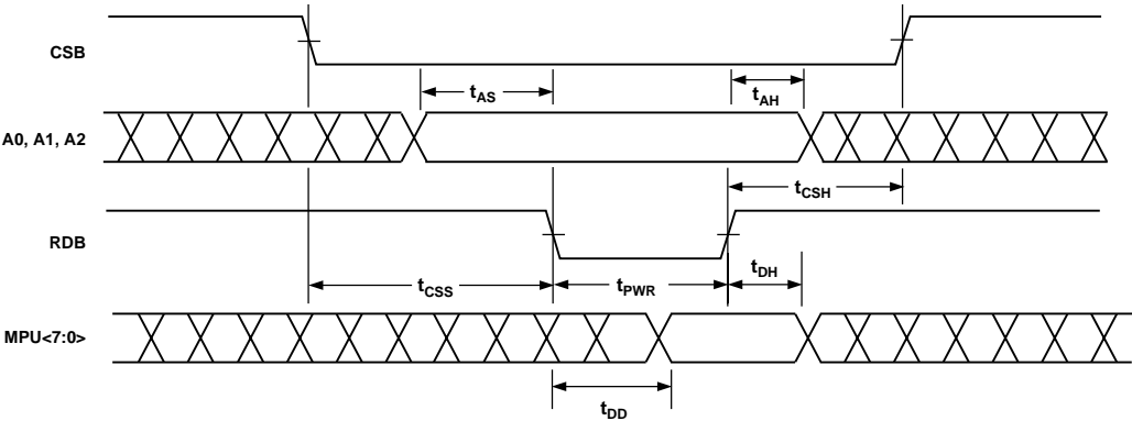
Figure 3. Read Timing
