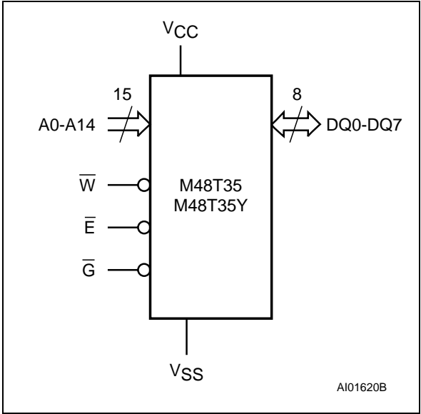
Figure 3. Logic Diagram
