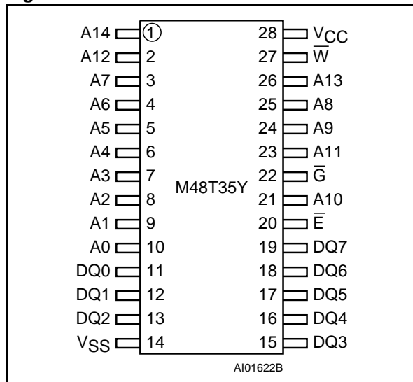
Figure 5. SOIC Connections
