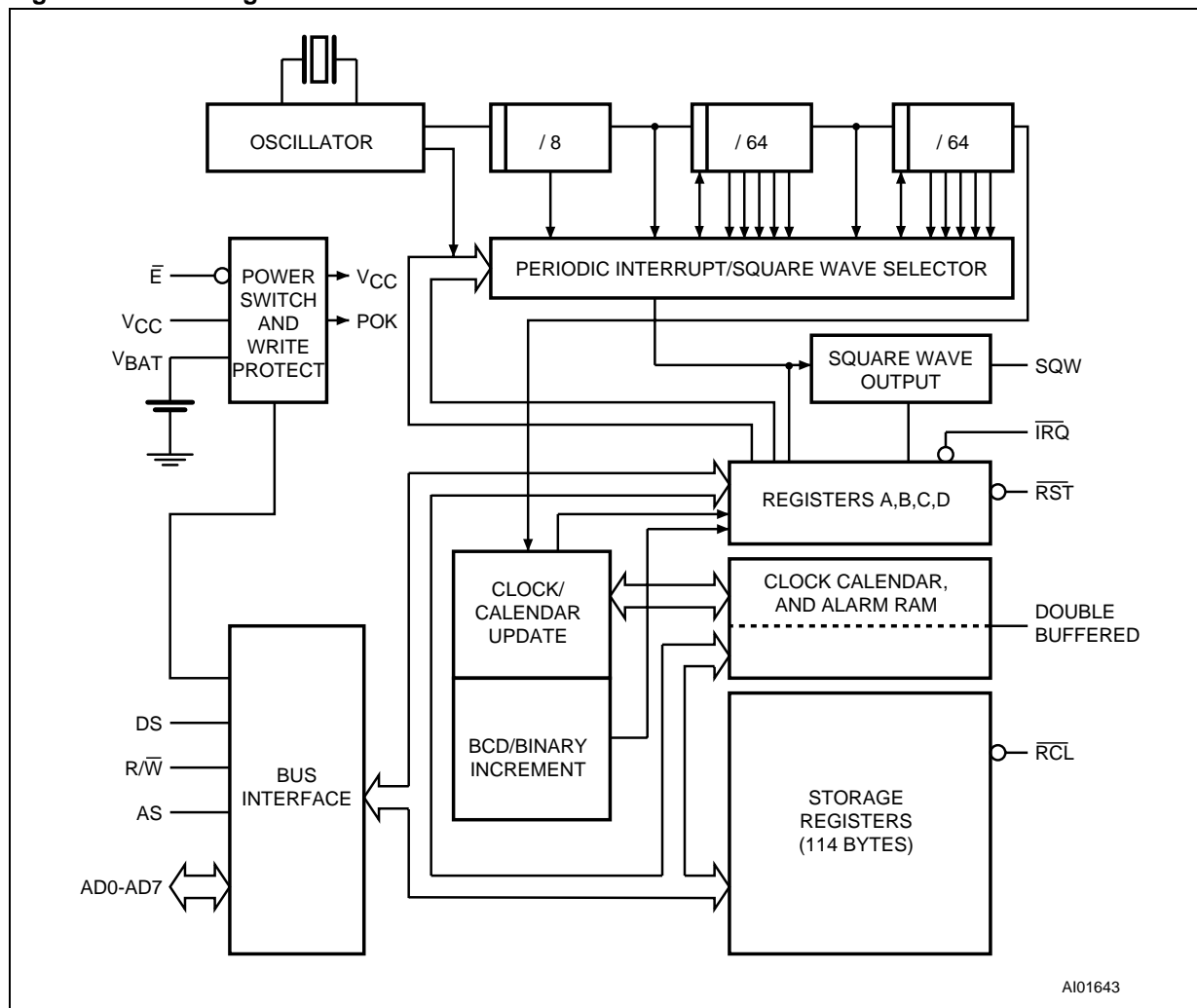
Figure 6. Block Diagram
