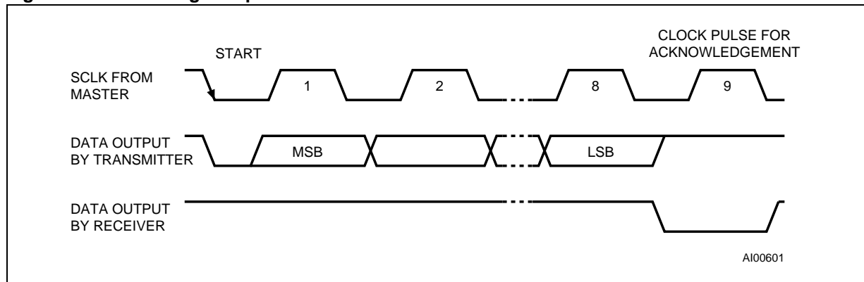
Figure 9. Acknowledge Sequence
