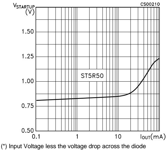
Figure 19: Minimum Input Voltage vs Output Current
