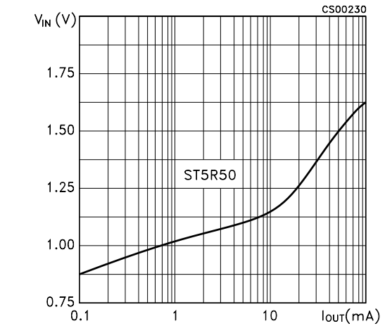
Figure 19: Minimum Input Voltage vs Output Current
