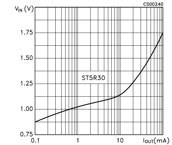
Figure 20: Minimum Input Voltage vs Output Current
