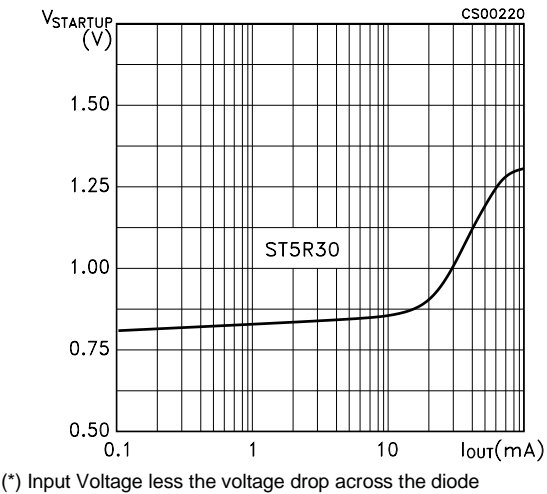
Figure 20: Minimum Input Voltage vs Output Current
