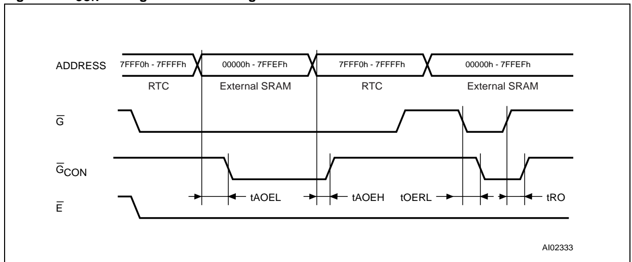
Figure 6. \overline{G}_{CON} Timing When Switching Between RTC and External SRAM
