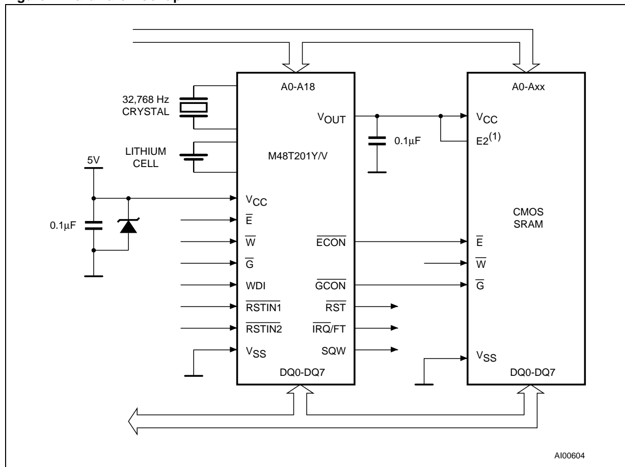
Figure 4. Hardware Hookup
