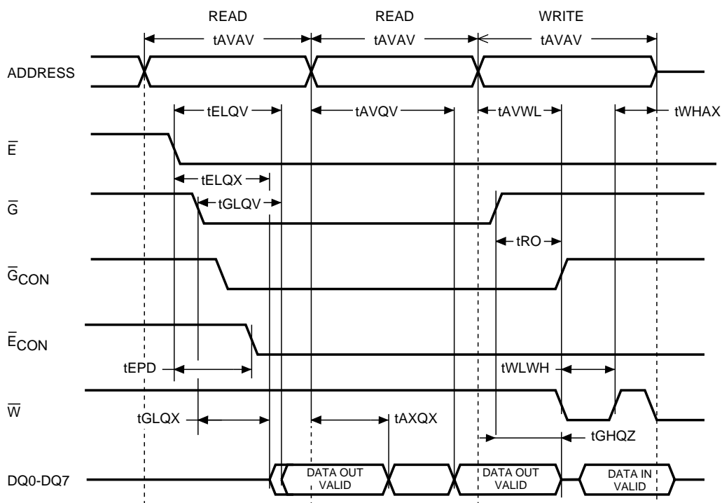
Figure 7. READ Cycle Timing: RTC and External RAM Control Signals
