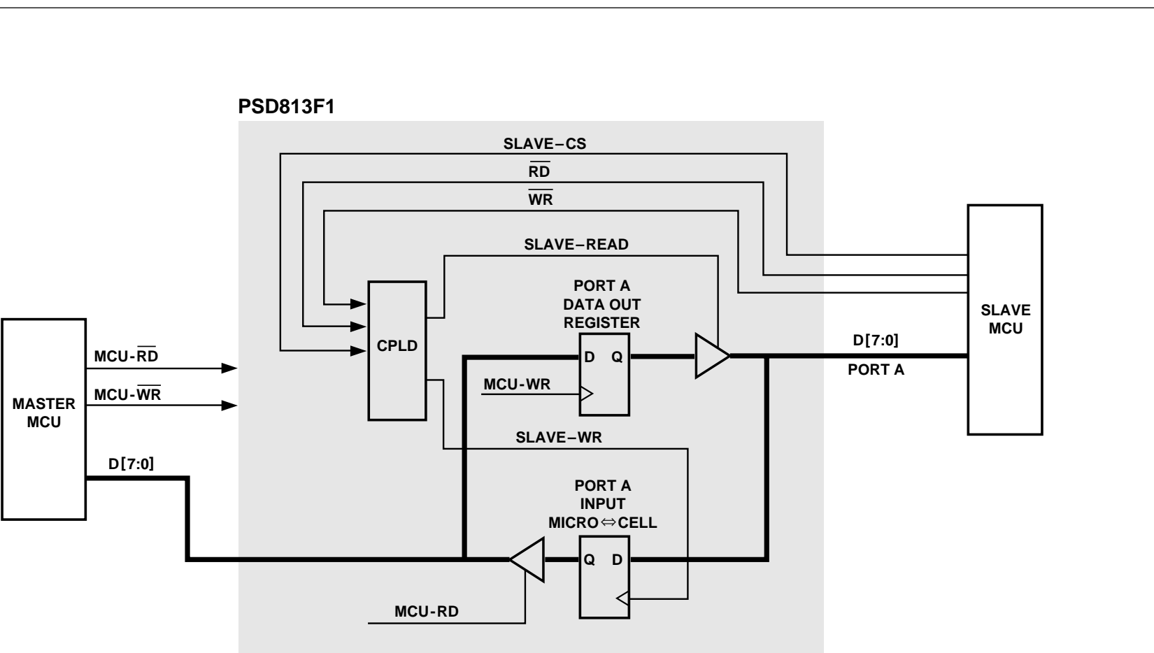
Figure 16. Handshaking Communication Using Input Micro⇌Cells
