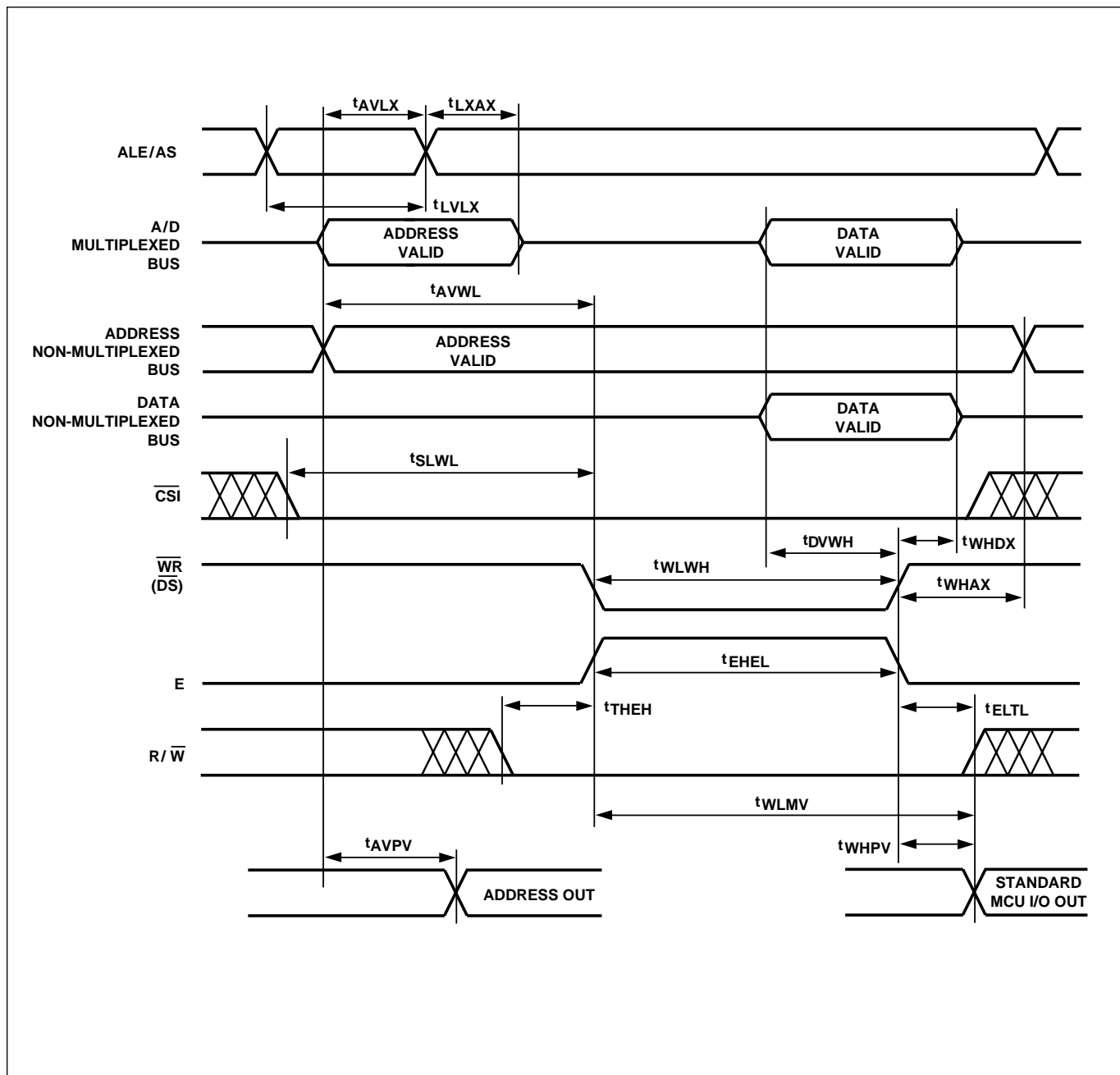
Figure 29. Write Timing
