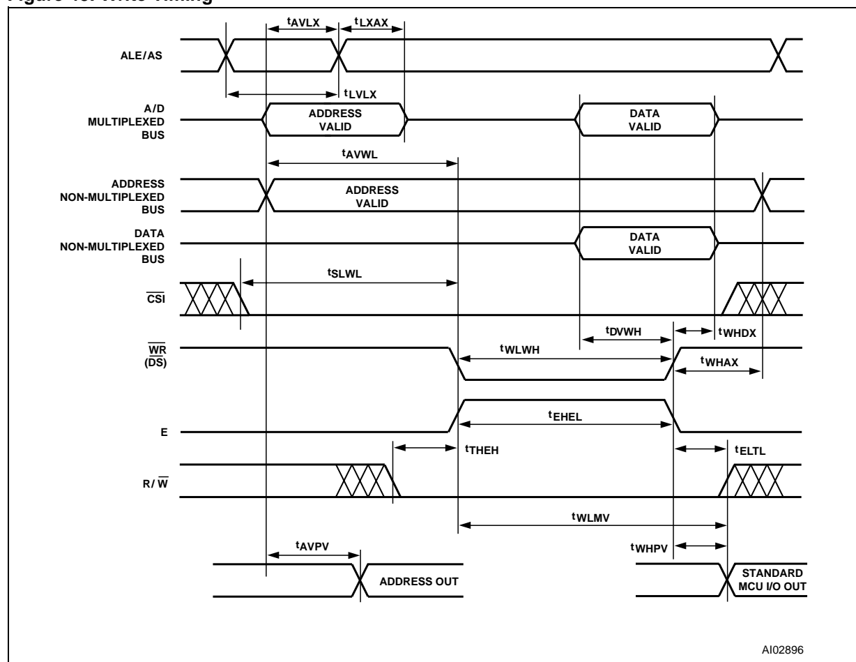
Figure 45. Write Timing
