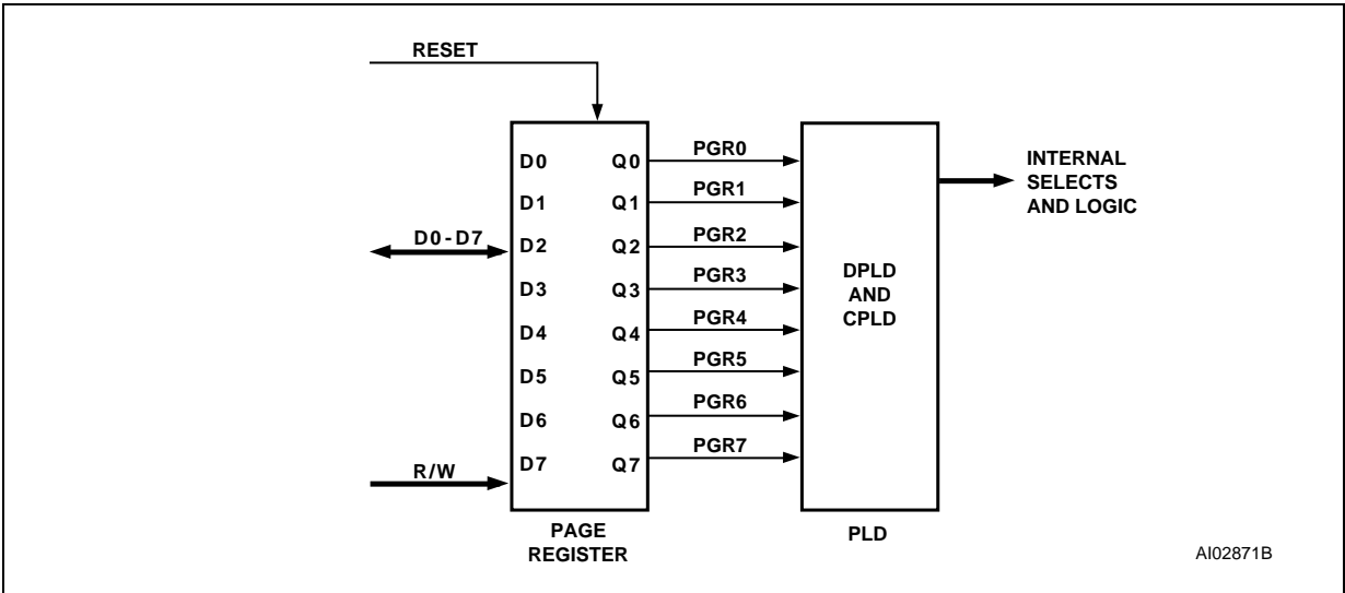
Figure 11. Page Register
