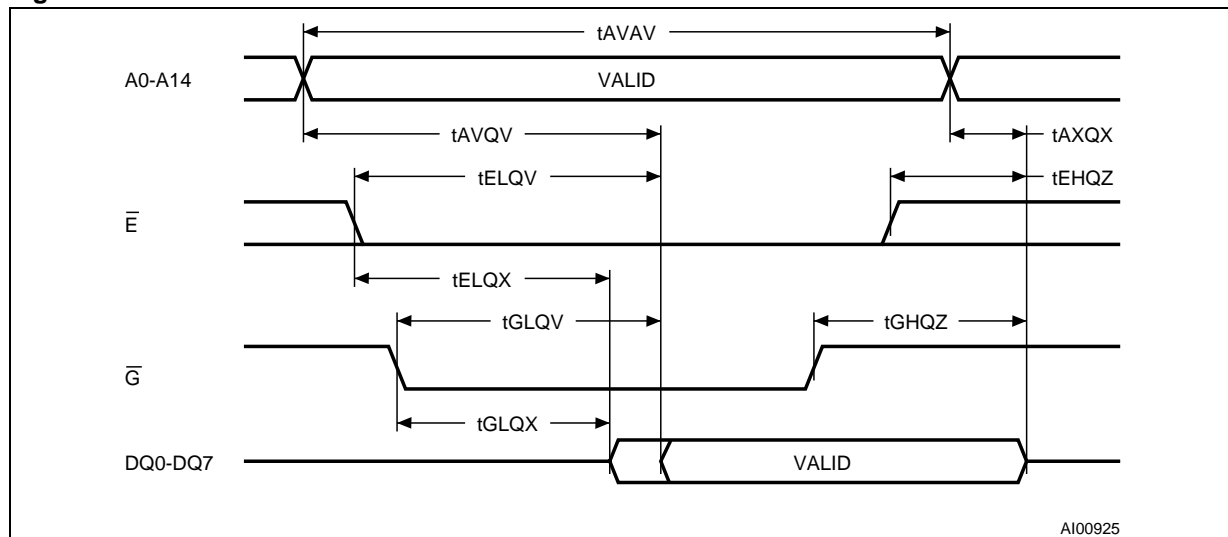
Figure 6. READ Mode AC Waveforms
