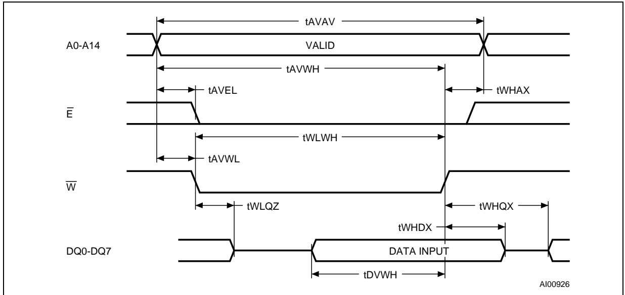
Figure 7. WRITE Enable Controlled, WRITE AC Waveform
