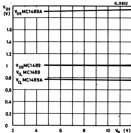
Figure 11 :Input Threshold versus Power Supply Volt
