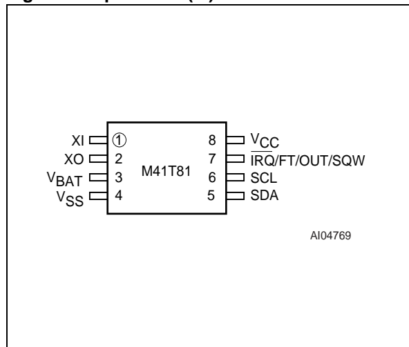
Figure 4. 8-pin SOIC (M) Connections
