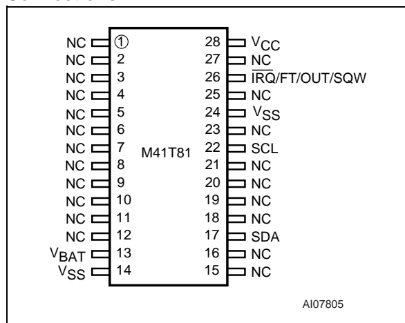
Figure 5. 28-pin, 300mil SOIC (MX) Connections
