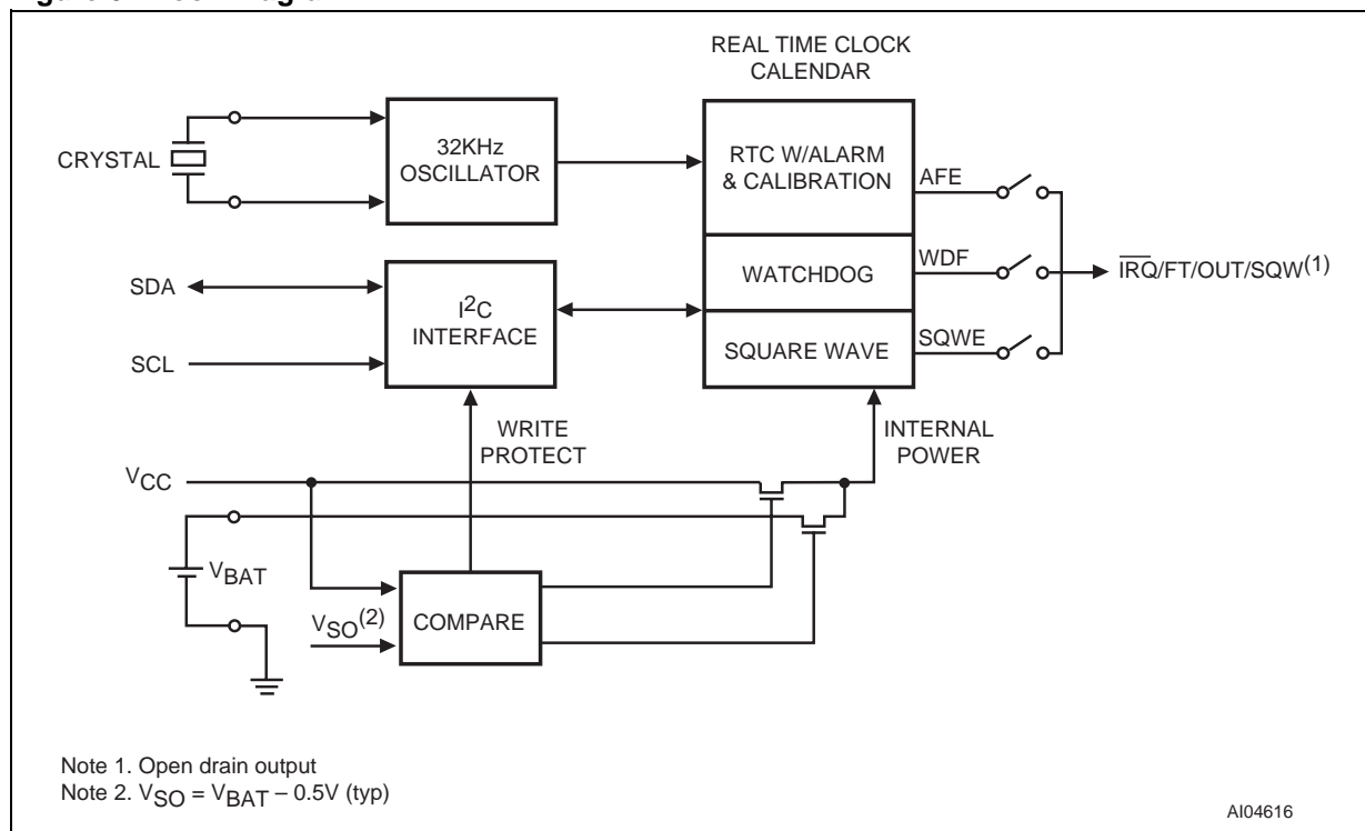
Figure 6. Block Diagram
