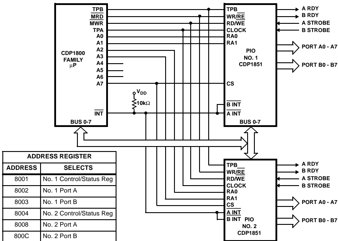
FIGURE 2. MEMORY SPACE I/O. THIS CONFIGURATION ALLOWS UP TO FOUR CDP1851s TO OCCUPY MEMORY SPACE 8XXX WITH NO ADDITIONAL HARDWARE (A4-A5 AND A6-A7 ARE USED AS RAO AND RA1 ON THE THIRD AND FOURTH PIO's)
