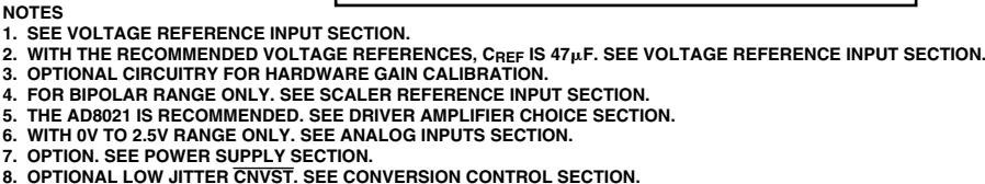
Figure 5. Typical Connection Diagram ( \pm 10 V Range Shown)
