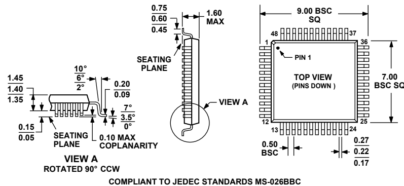
Figure 44. 48-Lead Quad Flatpack [LQFP] (ST-48) (Dimensions shown in millimeters)
