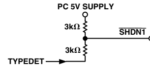
Figure 2. Using \overline{\text{SHDN1}} with TYPEDET Signal
