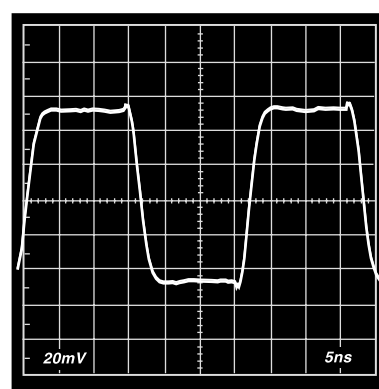
Figure 8.* 100 mV Step Response; G = -1 , V_S = \pm 2.5 \text{ V} or \pm 5 \text{ V}
