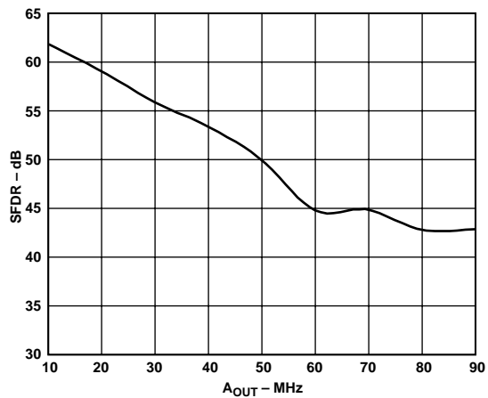
Figure 4. Wideband SFDR (200 MHz Clock) vs. A_{OUT} Frequency
