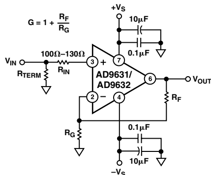
Figure 3. Noninverting Operation
