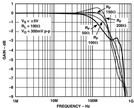
TPC 13. AD9631 Small Signal Frequency Response, G = +1
