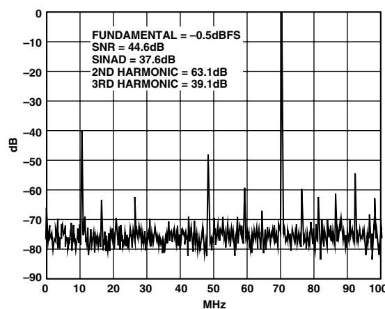
TPC 18. Spectrum: f_S = 140 MSPS, f_{IN} = 70.3 MHz
