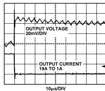
Figure 9. Load Transient Response, 19A–1A of Figure 2 Circuit
