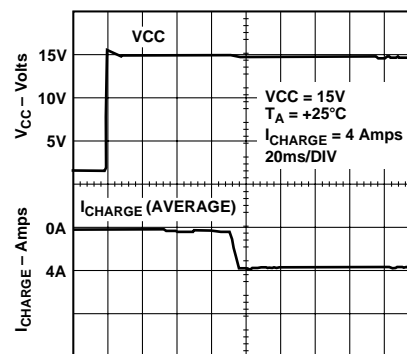
Figure 28. Source Current Due to Input Turn-On
