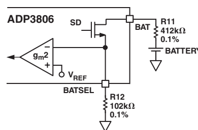
Figure 2. Battery Sense Disconnect Circuit
