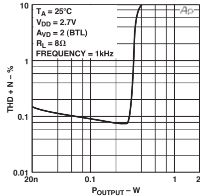
TPC 20. THD+N vs. P_{OUTPUT}
