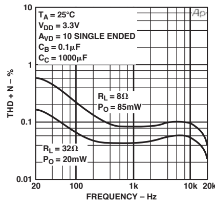
TPC 23. THD+N vs. Frequency
