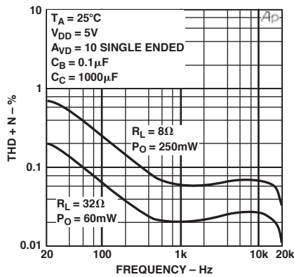
TPC 22. THD+N vs. Frequency
