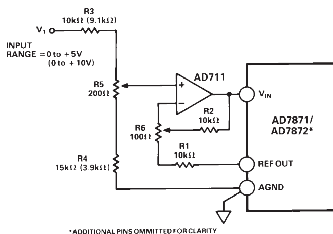
Figure 7. Unipolar Circuit
