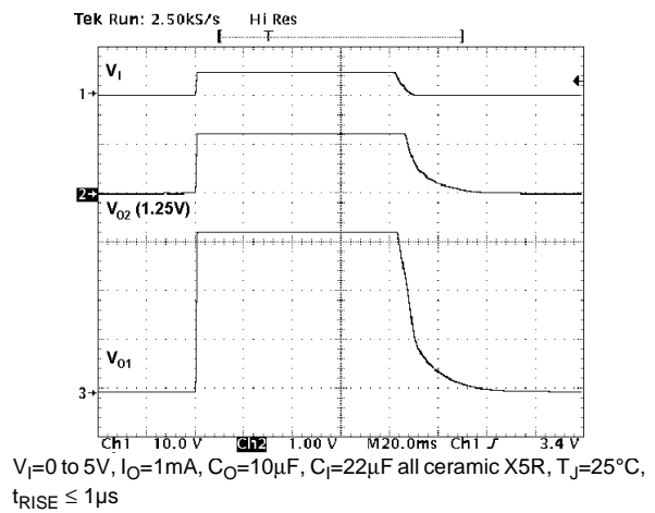
Figure 28 : Start-Up Transient
