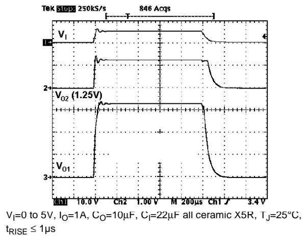
Figure 28 : Start-Up Transient
