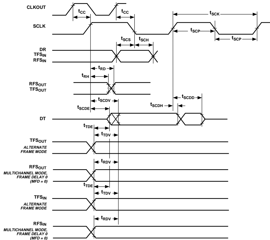
Figure 14. Serial Ports
