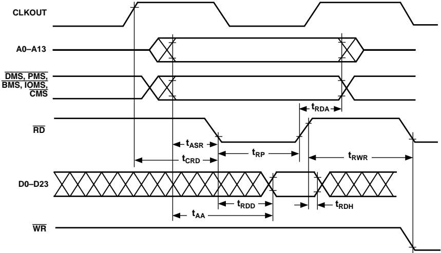
Figure 12. Memory Read
