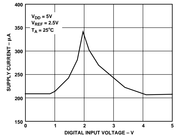
Figure 10. Supply Current vs. Digital Input Voltage
