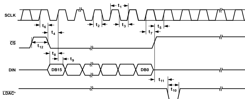
Figure 1. Timing Diagram
