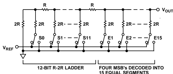
Figure 18. DAC Architecture
