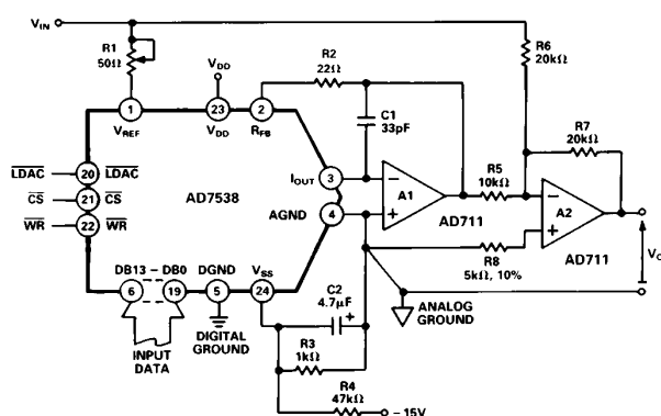
Figure 5. Bipolar Operation
