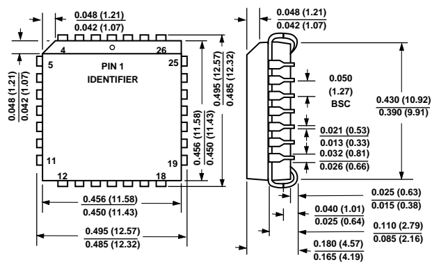
28-Pin LCC Package (Suffix E)
