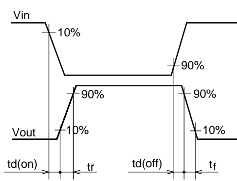
Waveform
