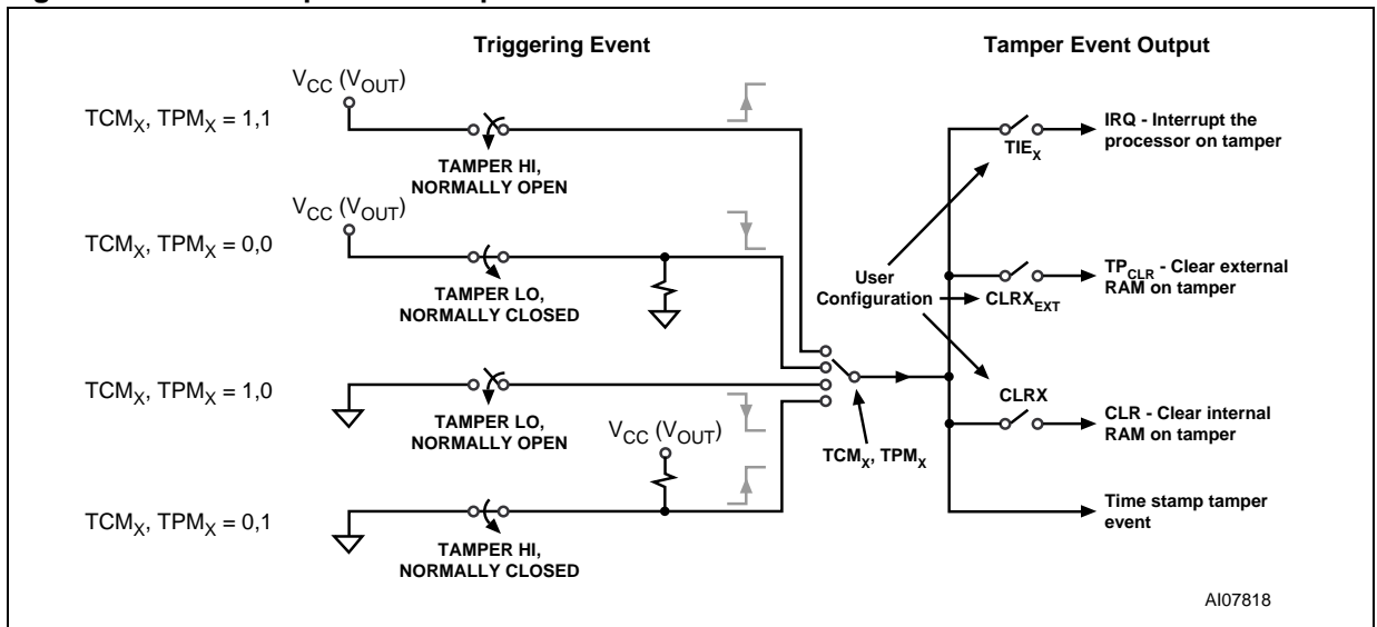
Figure 17. Basic Tamper Detect Options
