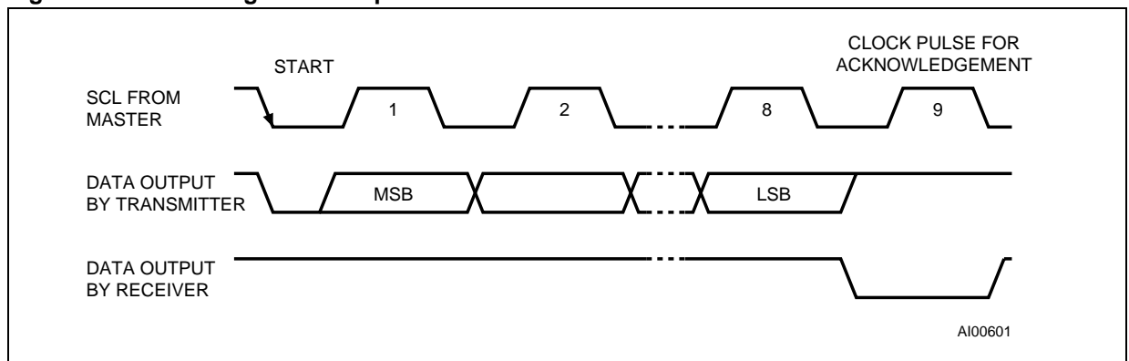
Figure 8. Acknowledgement Sequence
