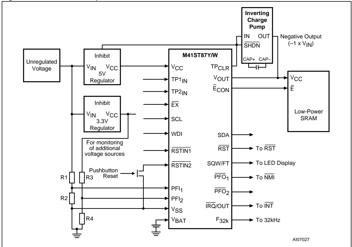
Figure 5. Hardware Hookup
