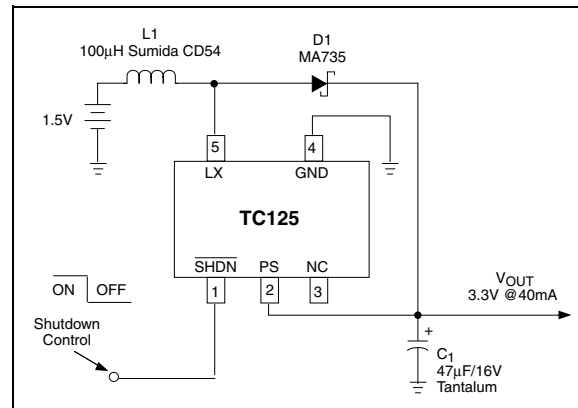
FIGURE 3-1: TYPICAL TC125 CIRCUIT
