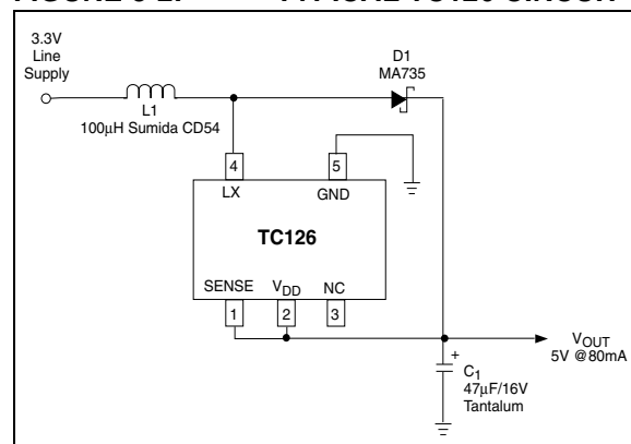
FIGURE 3-2: TYPICAL TC126 CIRCUIT
