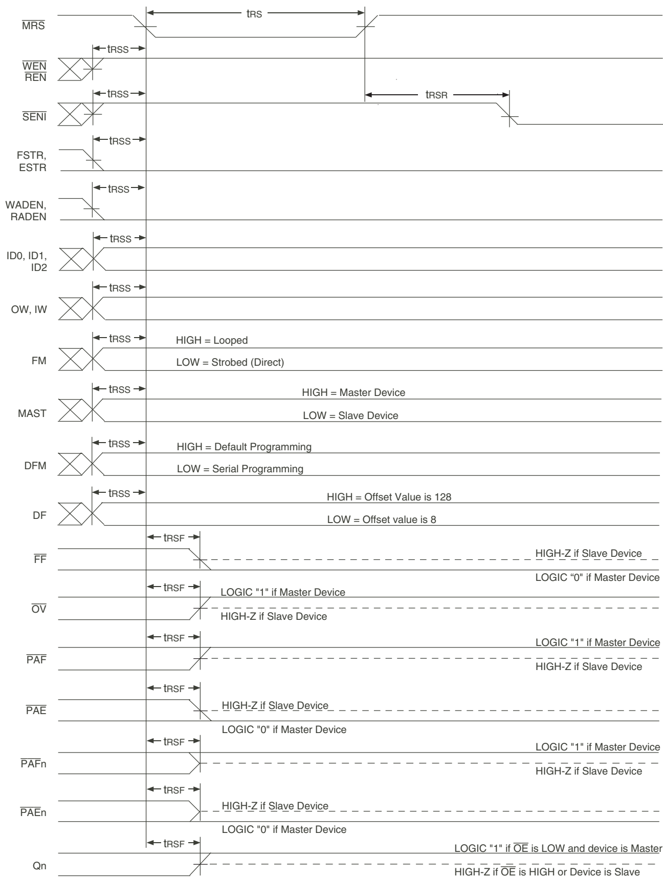
Figure 4. Master Reset
