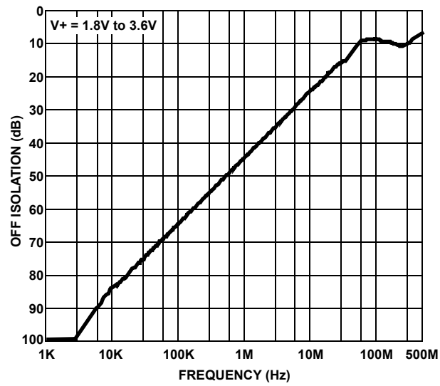
FIGURE 15. OFF ISOLATION
